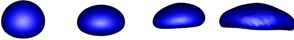
Fig. 22. Flattening of the droplet with increasing equivalent diameter. From left to right D_e = 3, 4.6, 6.4 and 8 mm.
