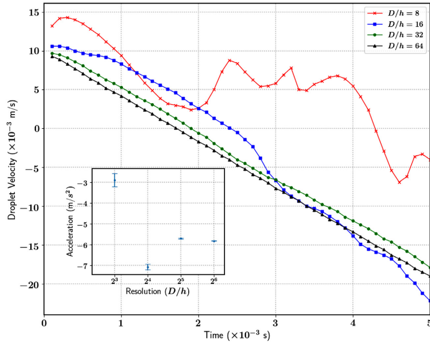
Fig. 30. Droplet velocity as a function of time, for different droplet resolutions D/h . The droplet velocity corresponds to that of the center of mass. Inset: convergence of the droplet acceleration as a function of its resolution, computed with the best linear fit over the temporal variation of the velocity. The error bar signifies the asymptotic standard error (least-squares) corresponding to the linear fit.
