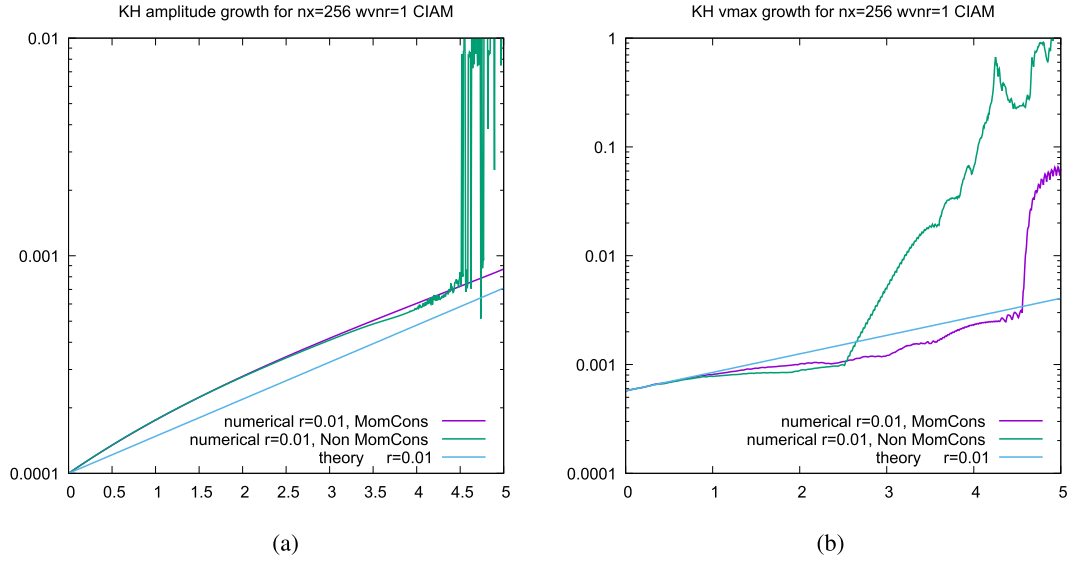
Fig. 14. Comparison of the theoretical and numerical growth for a boundary layer in the gas as a function of time with n_x = 256 grid points, a/h \simeq 6 points in the boundary layer, shift \Delta z = h/2 and U\tau/h = 0.08 : (a) amplitude plot; (b) maximum velocity plot.
